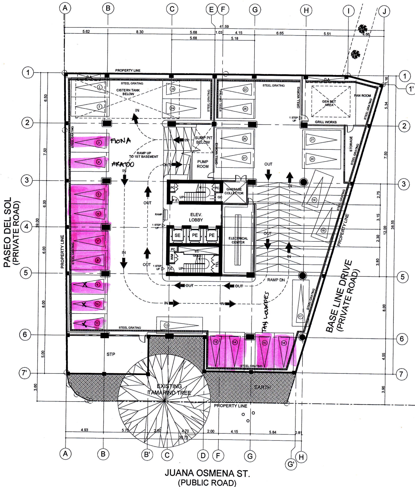
BASEMENT 2 FLOOR PLAN SCALE 1:200 MTS.
